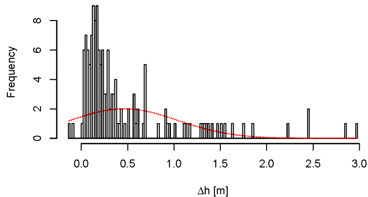
Figure 8. Histogram of the error distribution in “Test 2” / raw data. Superimposed is the normal distribution curve.
