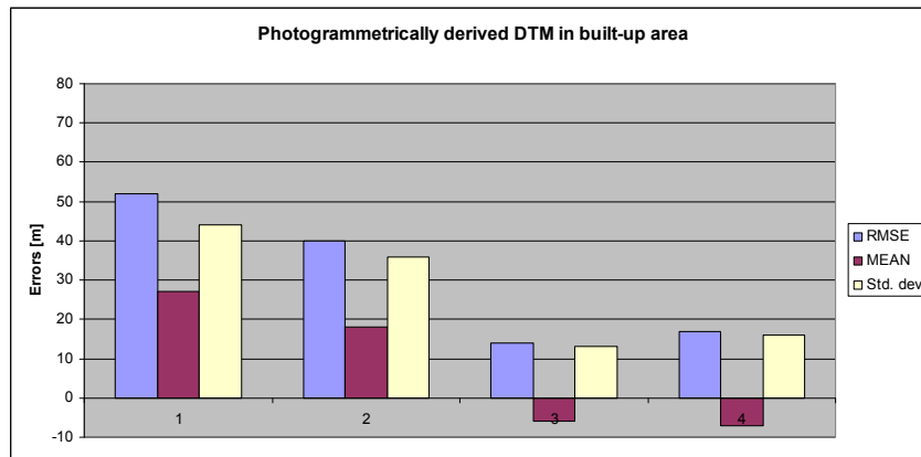
Figure 6. Results of DTM derivation by photogrammetry (standard accuracy measures) – “Test 1”. It means: 1...raw data ( n=146 , N=4 ), 2...editing based on precision (107, 3), 3...with filtering (56, 1), 4...filtering and completion (146, 3).
