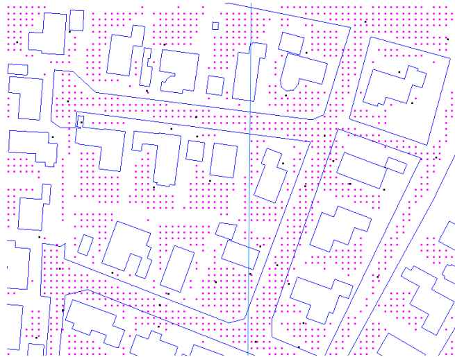
Figure 2. Result of the filtering and erasing of points within the outlines of buildings. It means: Remaining elevation points (pink), check points (black), buildings (blue).
