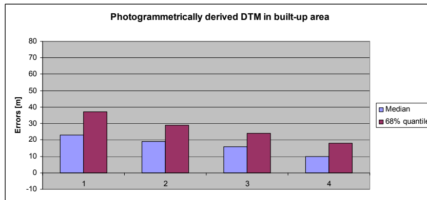
Figure 11. Results of DTM derivation by photogrammetry - “Test 2” (robust accuracy measures). It means: 1...raw data (n=146, N=5), 2...editing based on GIS data (146, 3), 3...with filtering (146, 2), 4... editing based on GIS data + filtering (146, 0).
