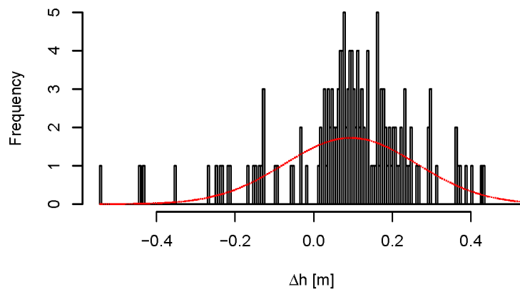
Figure 9. Histogram of the error distribution in “Test 2” / editing based on GIS data and filtering. Superimposed is the normal distribution curve.
