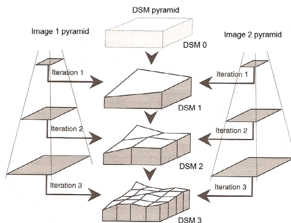
Figure 1. DSM generation by means of automated photogrammetry. Modified after Kraus (1996).
