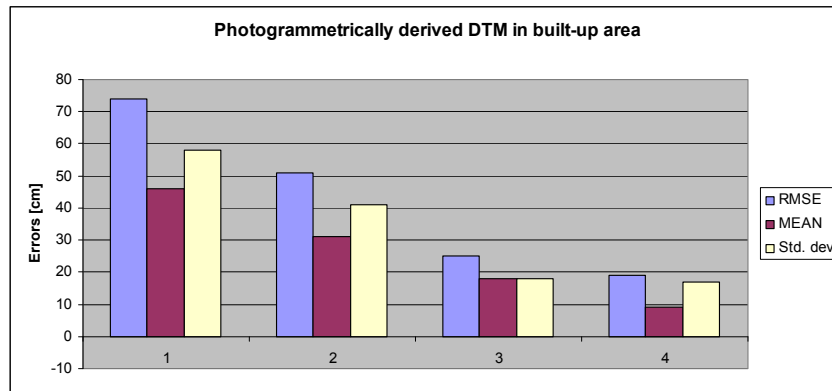
Figure 10. Results of DTM derivation by photogrammetry (standard accuracy measures) - “Test 2”. It means: 1...raw data (n=146, N=5), 2...editing based on GIS data (146, 3), 3...with filtering (146, 2), 4... editing based on GIS data+filtering (146, 0).
