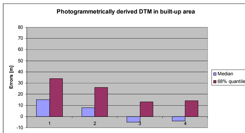
Figure 7. Results of DTM derivation by photogrammetry (robust accuracy measures) – “Test 1”. It means: 1...raw data ( n=146 , N=4 ), 2...editing based on precision (107, 3), 3...with filtering (56, 1), 4...filtering and completion (146, 3).
